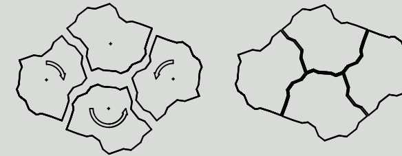
Basic laying pattern is created by using 4 stones rotated 90° to each other.
